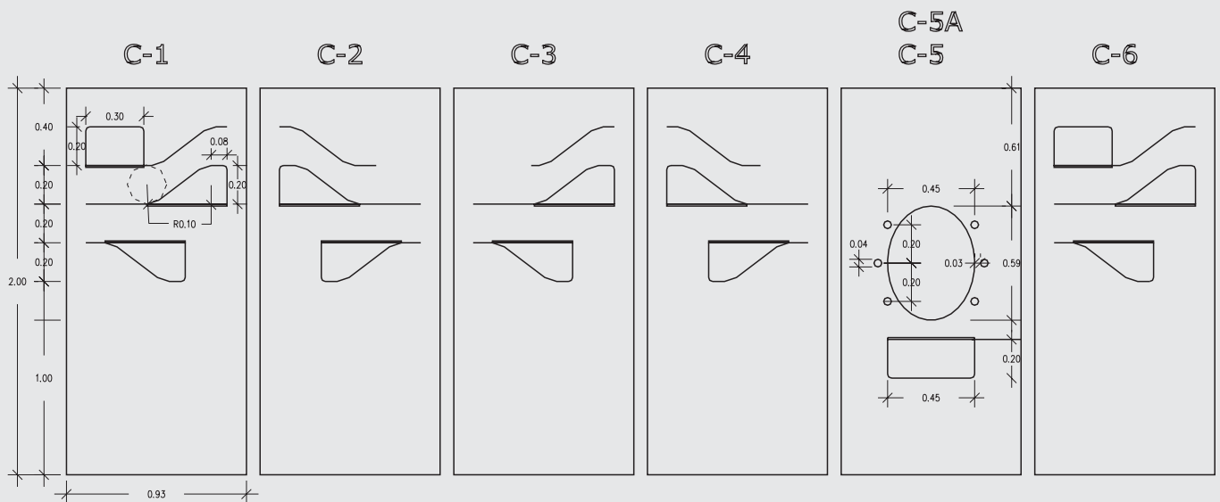
Detail drawings of holes of partition panels by Corian
